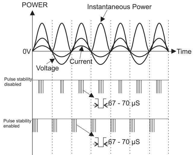
Figure 9: LED pulse output in fast mode
