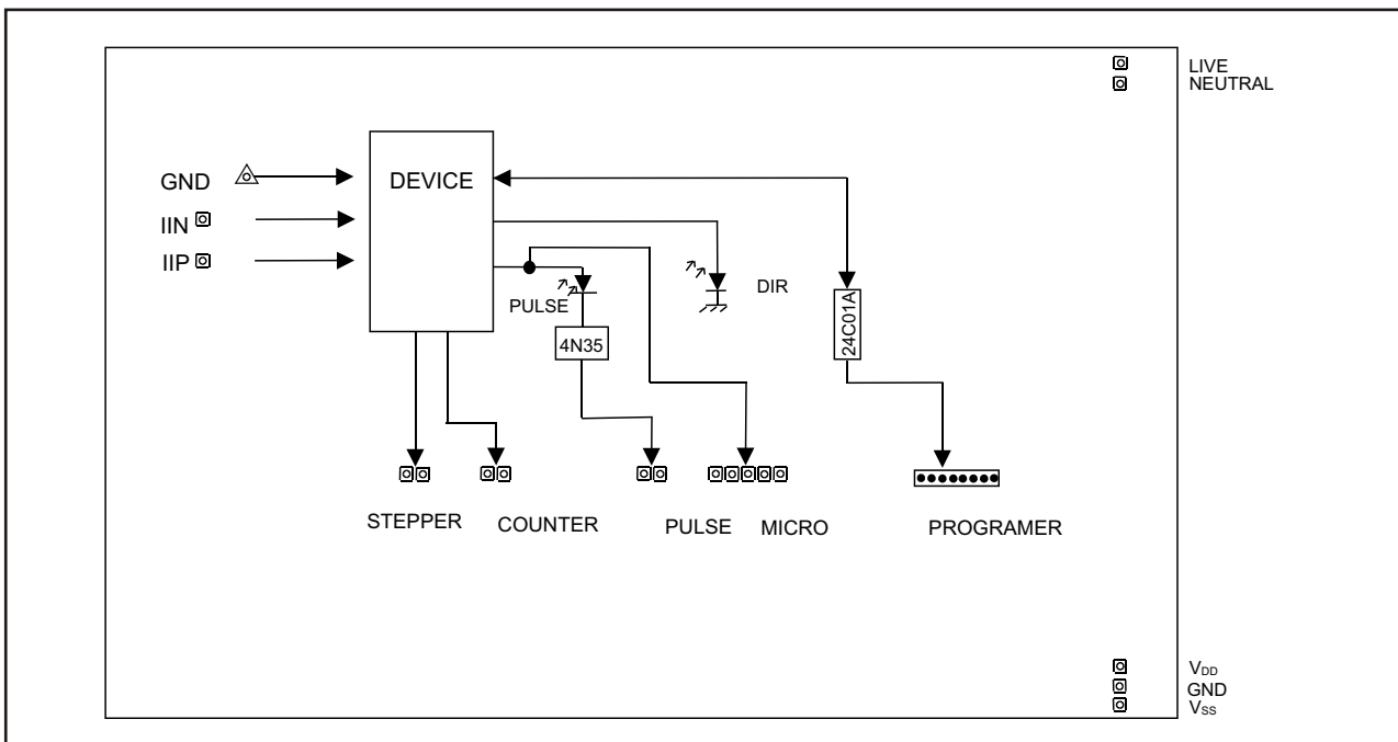
Figure 1: Functional Diagram
